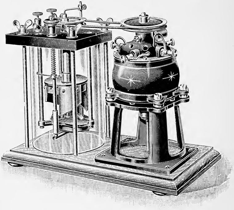
FIG. 26.—MERCURY JET INTERRUPTER.
